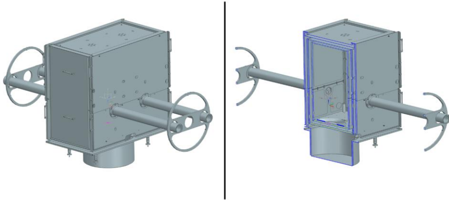
Figure 1 CAD view of the Cryogenic Shield Assembly
