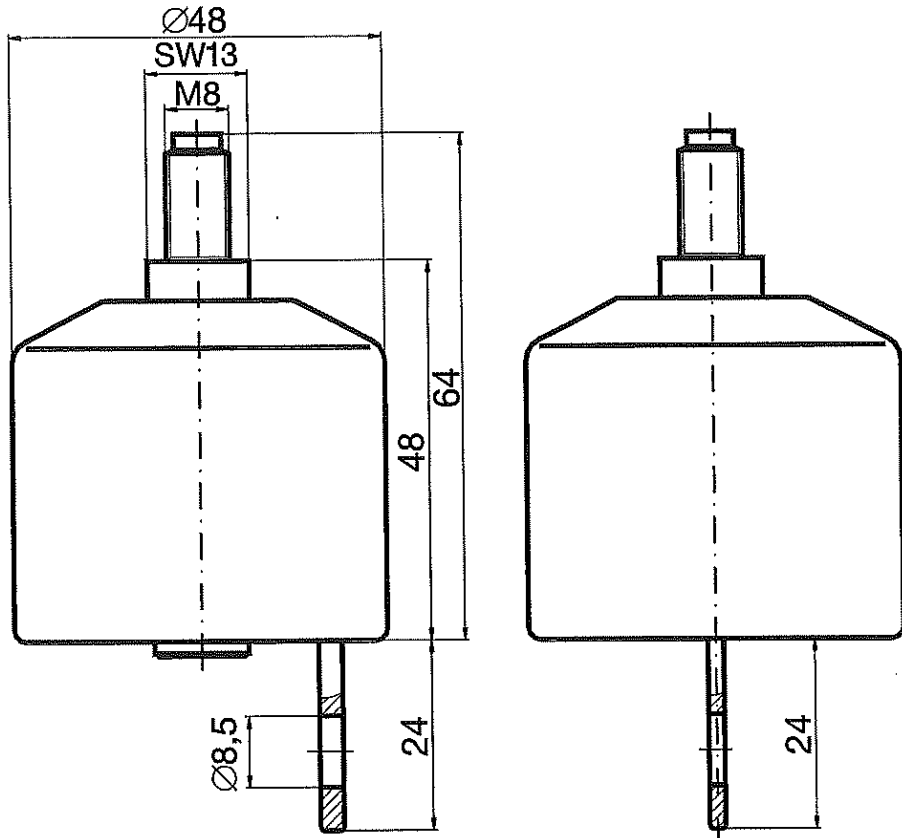
2 - surge arrester without disconnector
