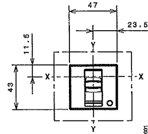
A=79 3-4 POLES
