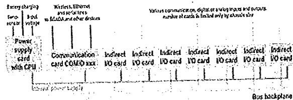
RTU7M internal architecture from 2017
