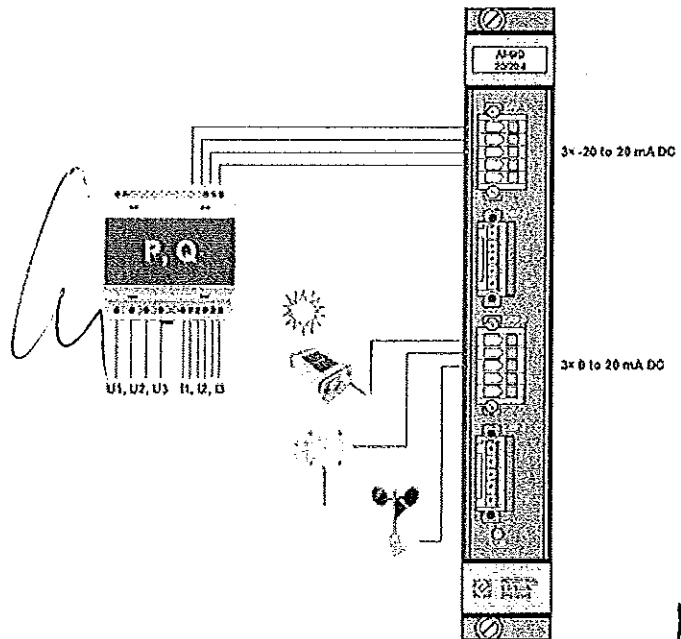
Example of connection of card AI-6ID with different measuring ranges of input groups
