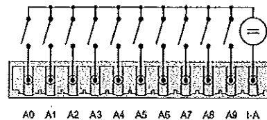
Passive inputs connection
