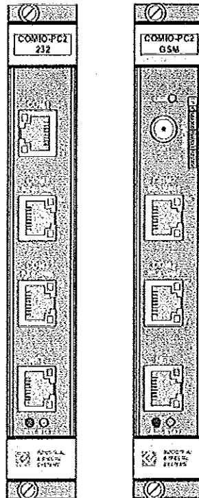
Front panels with connectors of cards COMIO-PC2
