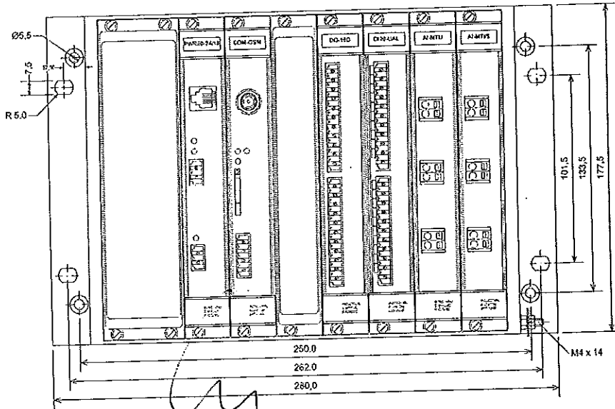
Dimensions of chassis with 8 slots
