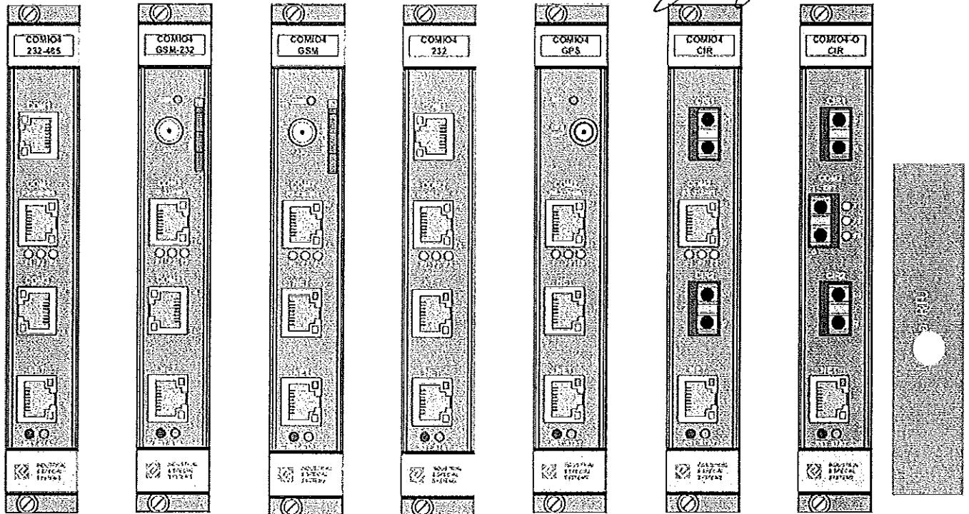
Front panels with connectors of cards COMIO4
